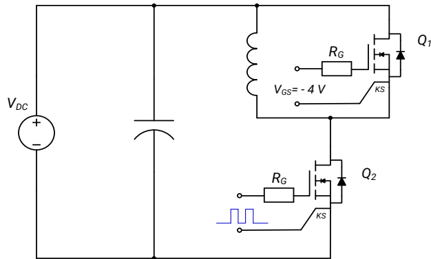
Figure 30. Clamped Inductive Switching Waveform Test Circuit
