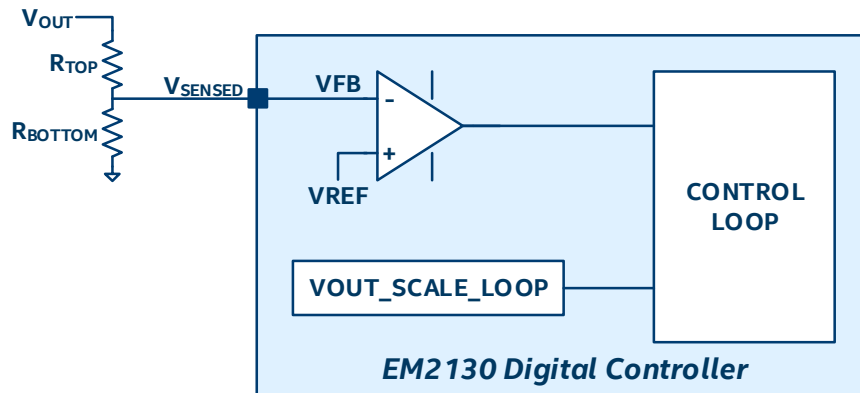
Figure 5: V OUT Scaling Diagram
