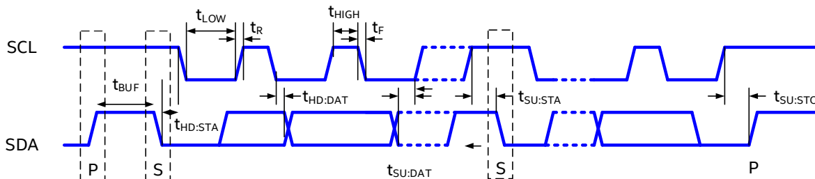
Figure 1: PMBus Timing Diagram
