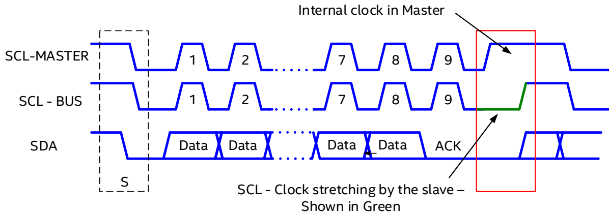
Figure 2: Example of Periodic & Random Clock Stretching
