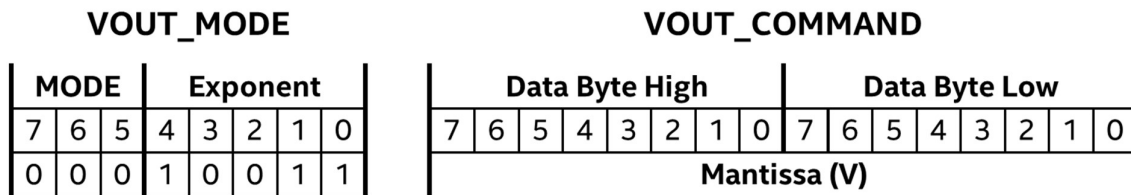
Figure 4: Data Byte Structure, VOUT_MODE and VOUT_COMMAND
