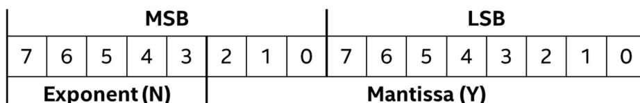
Figure 3: Linear Data Format
