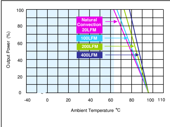
Figure 20: AEE00BB12-M Derating Curves (without heatsink) Vin = 12Vdc Load: Io = 0 to ±0.417
