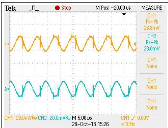
Figure 73: AEE00BB48-M Ripple and Noise Measurement Vin = 48Vdc Load: Io = ±0.417 Ch 1: Vo1 Ch 2: Vo2
