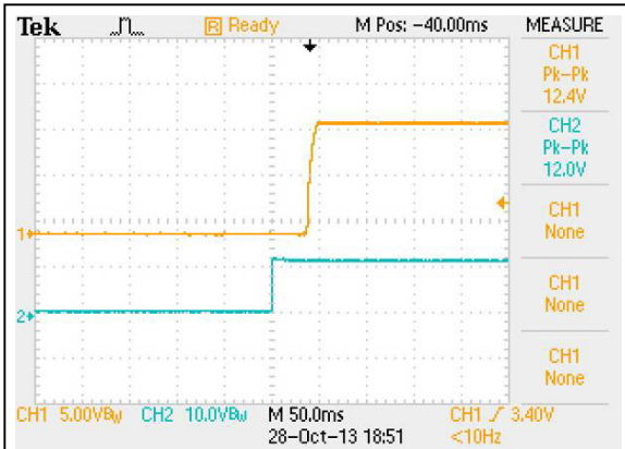
Figure 19: AEE00BB12-M Output Voltage Startup Characteristic by Vin Vin = 12Vdc Load: Io = ±0.417A Ch1: Vo1 Ch2: Vin
