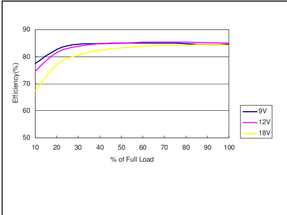
Figure 15: AEE00BB12-M Efficiency Versus Output Current Curve Vin = 9 to 18Vdc Load: Io = 0 to ±0.417A
