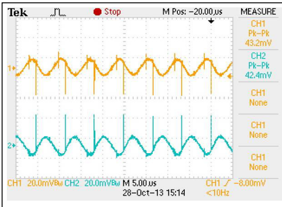
Figure 17: AEE00BB12-M Ripple and Noise Measurement Vin = 12Vdc Load: Io = ±0.417 Ch 1: Vo1 Ch 2: Vo2
