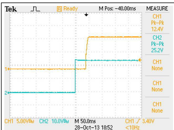
Figure 47: AEE00BB24-M Output Voltage Startup Characteristic by Vin Vin = 24Vdc Load: Io = ±0.417A Ch1: Vo1 Ch2: Vin
