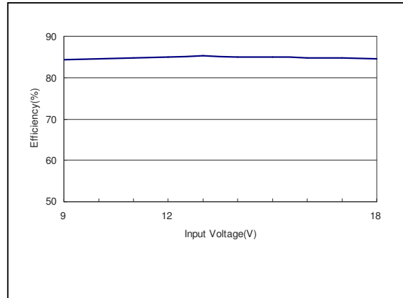
Figure 16: AEE00BB12-M Efficiency Versus Input Voltage Curve Vin = 9 to 18Vdc Load: Io = ±0.417
