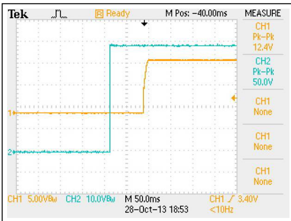
Figure 75: AEE00BB48-M Output Voltage Startup Characteristic by Vin Vin = 48Vdc Load: Io = ±0.417A Ch1: Vo1 Ch2: Vin
