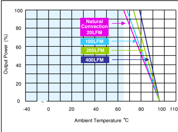
Figure 76: AEE00BB48-M Derating Curves (without heatsink) Vin = 48Vdc Load: Io = 0 to ±0.417
