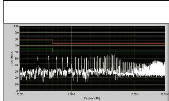
Figure 77: AEE00BB48-M Conduction Emission of EN550122 Class A Vin = 48Vdc Load: Io = 1 ±0.417
