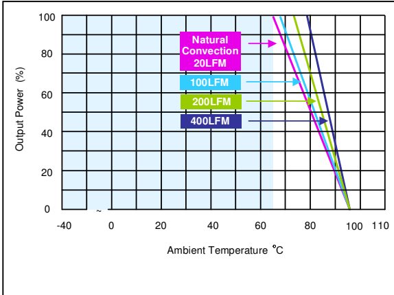
Figure 48: AEE00BB24-M Derating Curves (without heatsink) Vin = 24Vdc Load: Io = 0 to ±0.417
