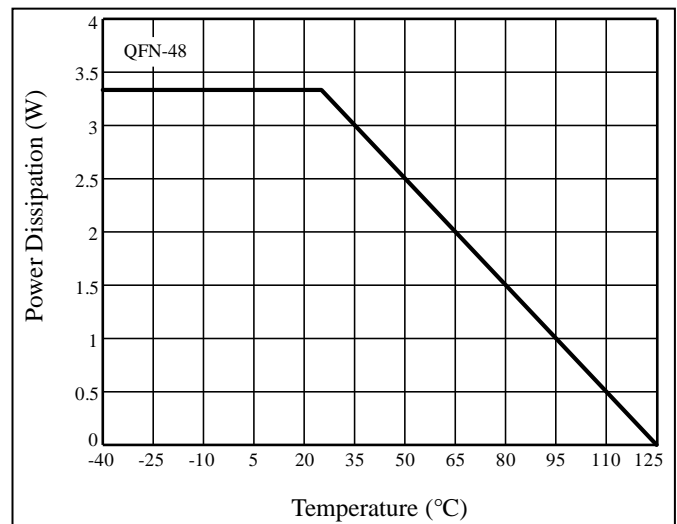
Figure 18 Dissipation Curve
