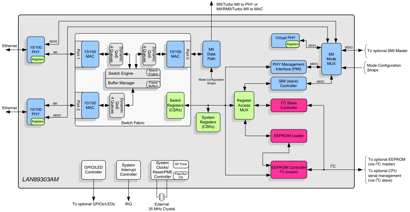
Figure 1 Internal Block Diagram
