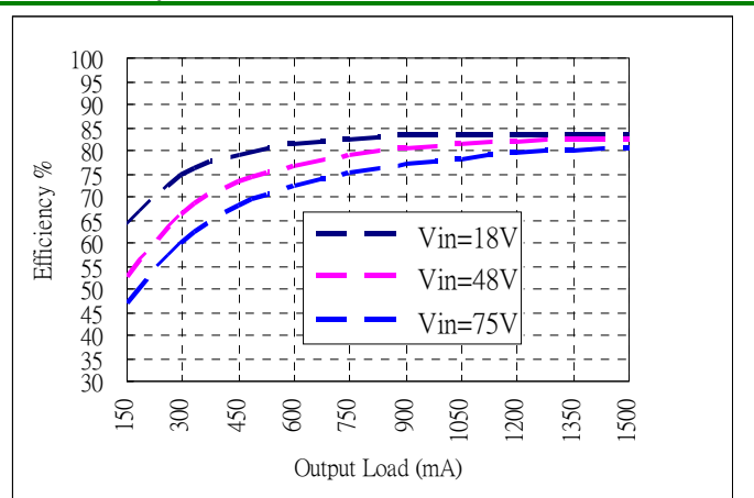
Efficiency vs. Load @ +25° Ambient, AEE01AA36-LS
