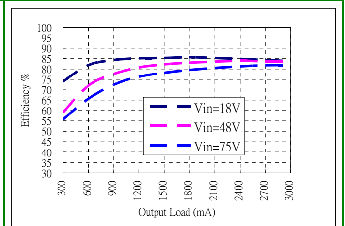
Efficiency vs. Load @ +25° Ambient, AEE03A36-LS
