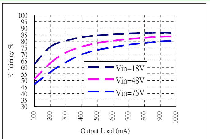
Efficiency vs. Load @ +25° Ambient, AEE01C36-LS
