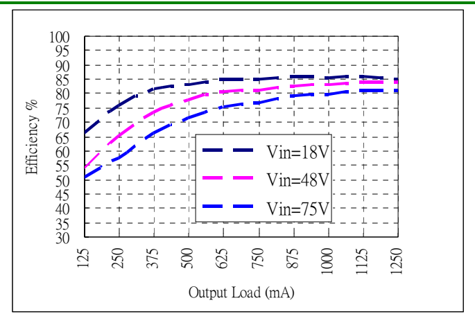
Efficiency vs. Load @ +25° Ambient, AEE01B36-LS
