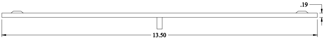
FRONT VIEW
