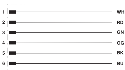
Contact assignment of the 7/8" plug
