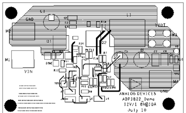
Figure 15. Bottom Layer
