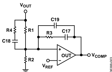
Figure 3. Compensation Circuit
