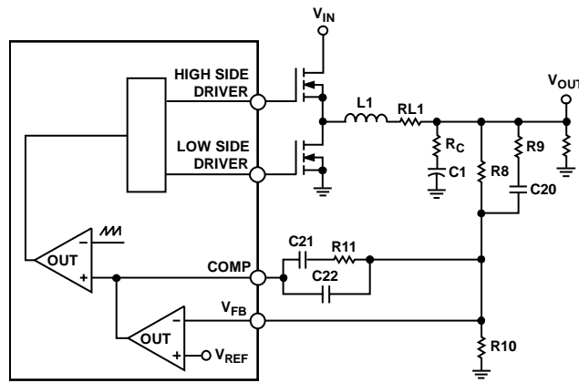
Figure 2. Control Loop
