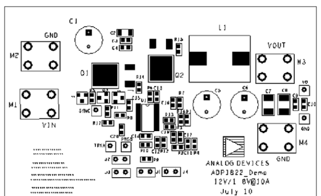
Figure 16. Silkscreen Top
