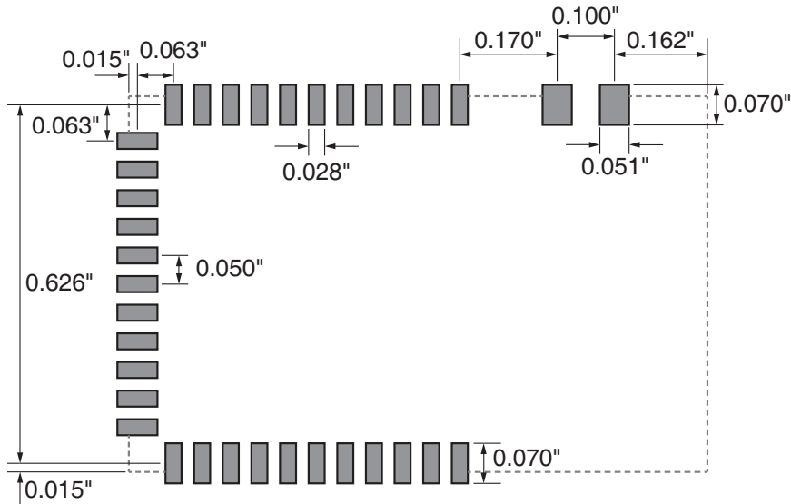
Figure 109: HUM-A-900-PRO-CAS Recommended PCB Layout
