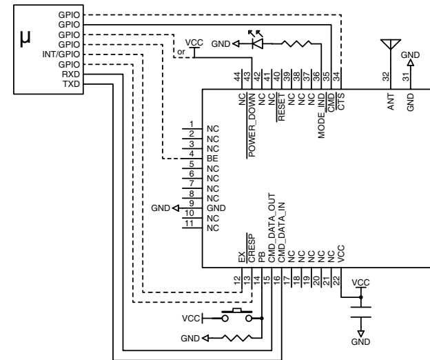
Figure 106: Amplified HumPRO™ Series Transceiver Basic Application Circuit
