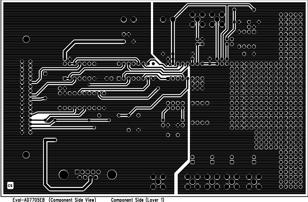
Fig. 15. The Evaluation Board Component Side Artwork.
