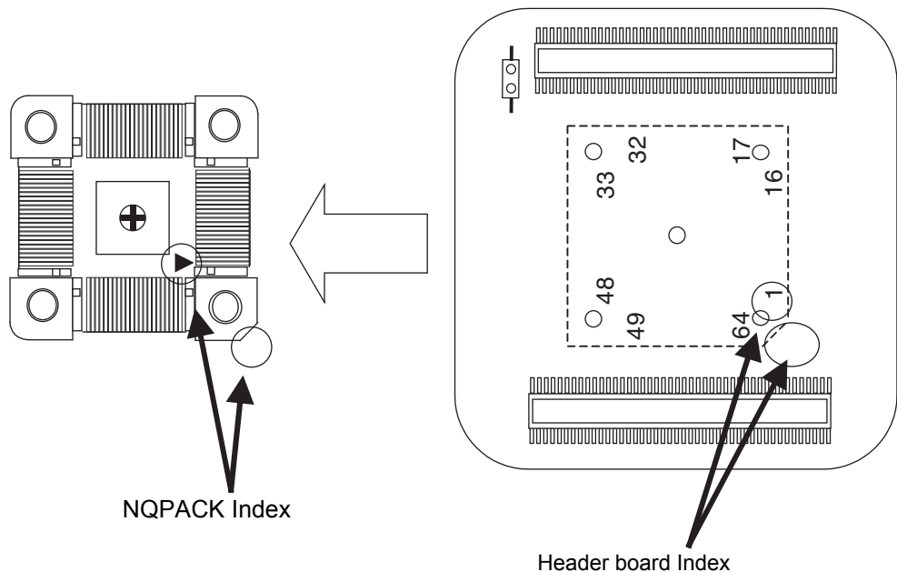
Figure 5-1. Index position
