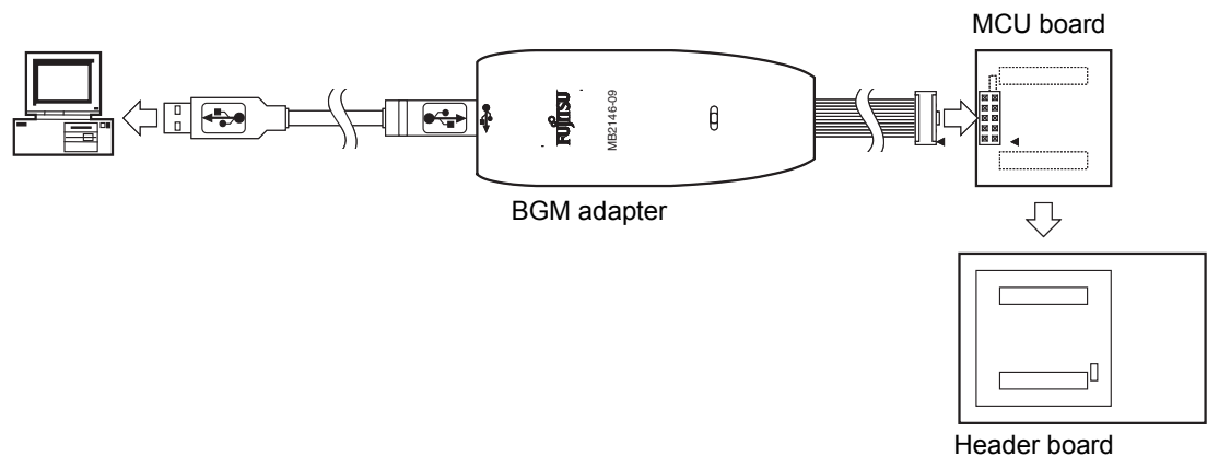
Figure 1-1. System-configuration
