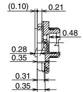
Y-Y cross section
