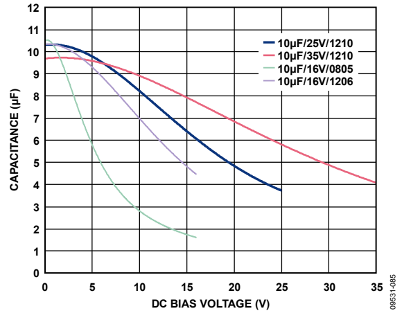
Figure 85. Capacitance vs. Voltage Characteristic Different Case Sizes
