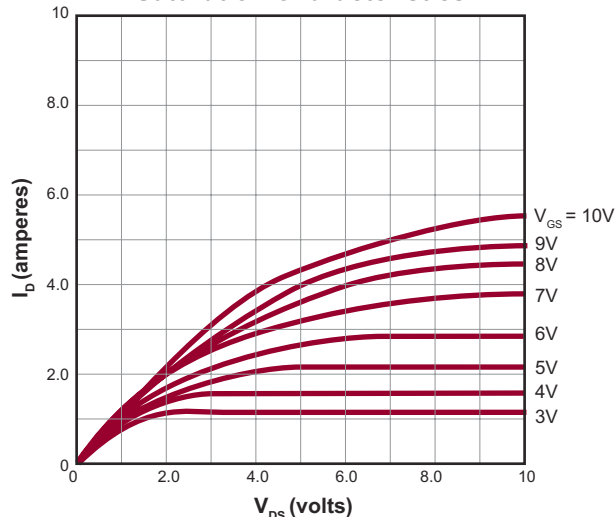
Saturation Characteristics
