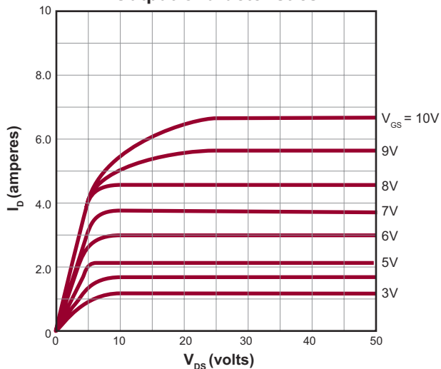
Output Characteristics
