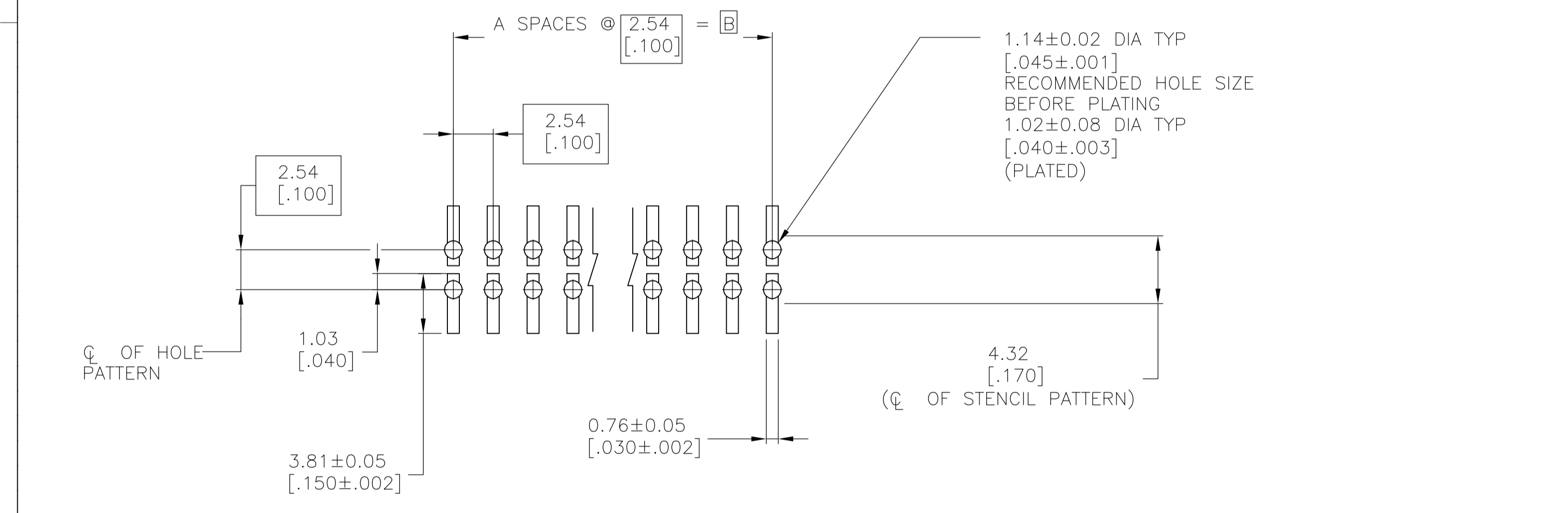
RECOMMENDED PC BOARD MOUNTING DIMENSIONS FOR .063[1.60] THICK PC BOARD AND .012[.305] STENCIL THICK
