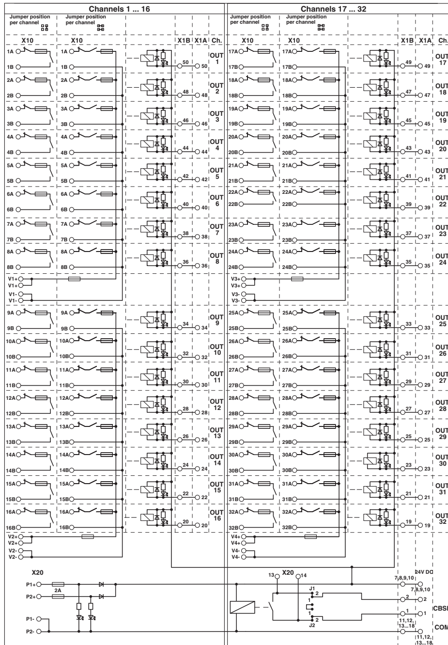
Circuit diagram
