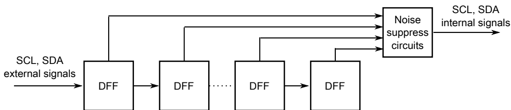
Figure 51-5. Programmable input glitch filter diagram
