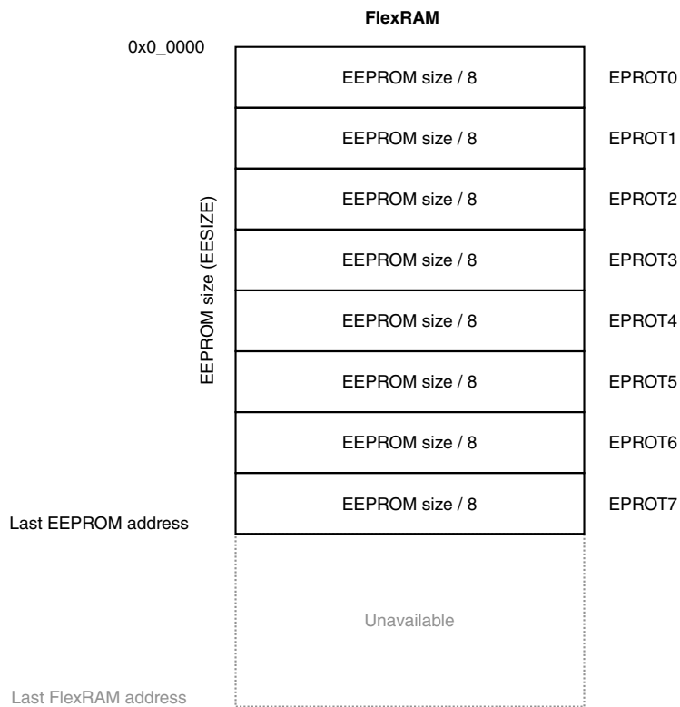
Figure 29-6. EEPROM protection
