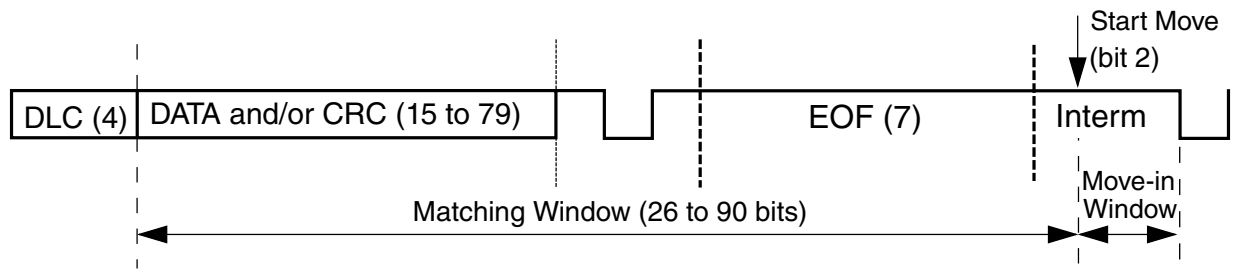
Figure 49-4. Matching and move-in time windows
