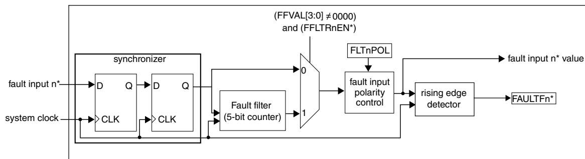
Figure 40-70. Fault input n control block diagram
