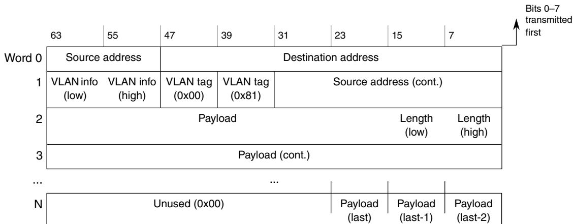
Figure 45-15. VLAN-tagged frame 64-bit mapping example
