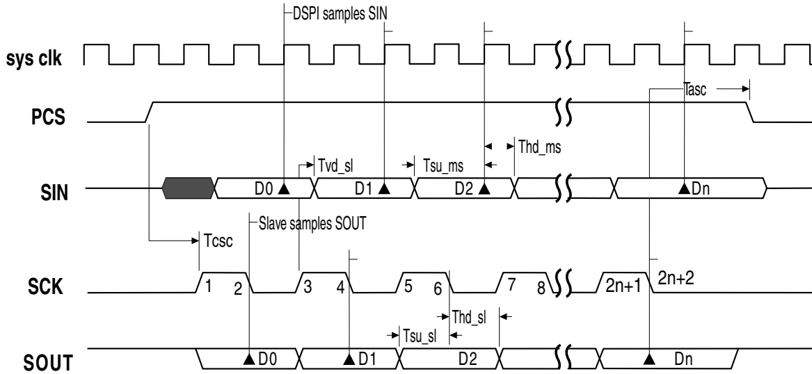
Figure 50-11. SPI Modified Transfer Format (MTFE=1, CPHA=1, f_{sck} = f_{sys}/2 )
