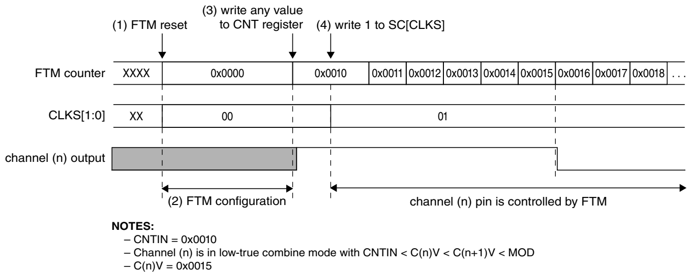
Figure 40-96. FTM behavior after reset when the channel (n) is in Combine mode
