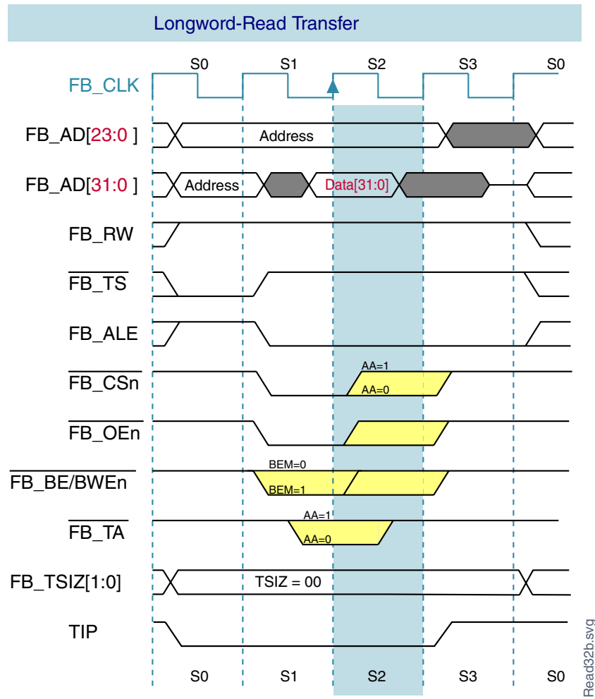
Figure 31-11. Longword-Read Transfer
