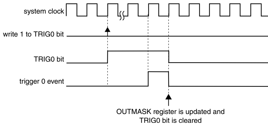
Figure 40-53. OUTMASK synchronization with ( \text{SYNCMODE} = 0 ), ( \text{HWTRIGMODE} = 0 ), ( \text{SYNCHOM} = 1 ), ( \text{PWMSYNC} = 0 ), and a hardware trigger was used
