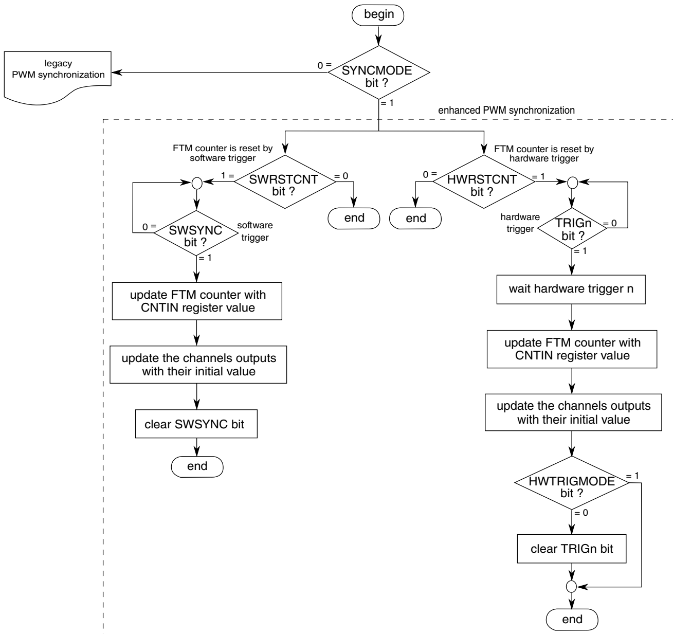
Figure 40-58. FTM counter synchronization flowchart
