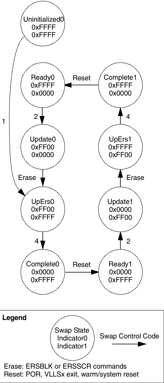
Figure 29-12. Valid Swap State Sequencing
