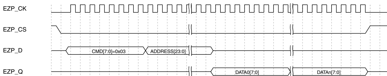
Figure 30-5. Read command sequence
