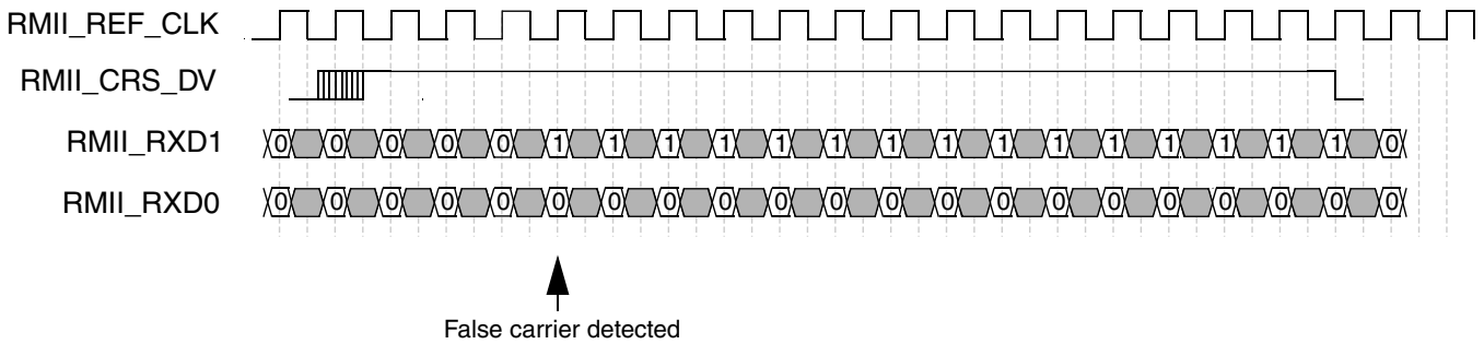
Figure 45-20. RMII receive operation with false carrier
