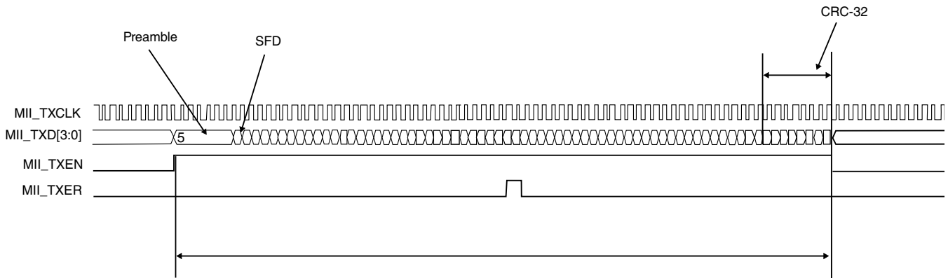
Figure 45-23. MII transmit operation — errored frame
