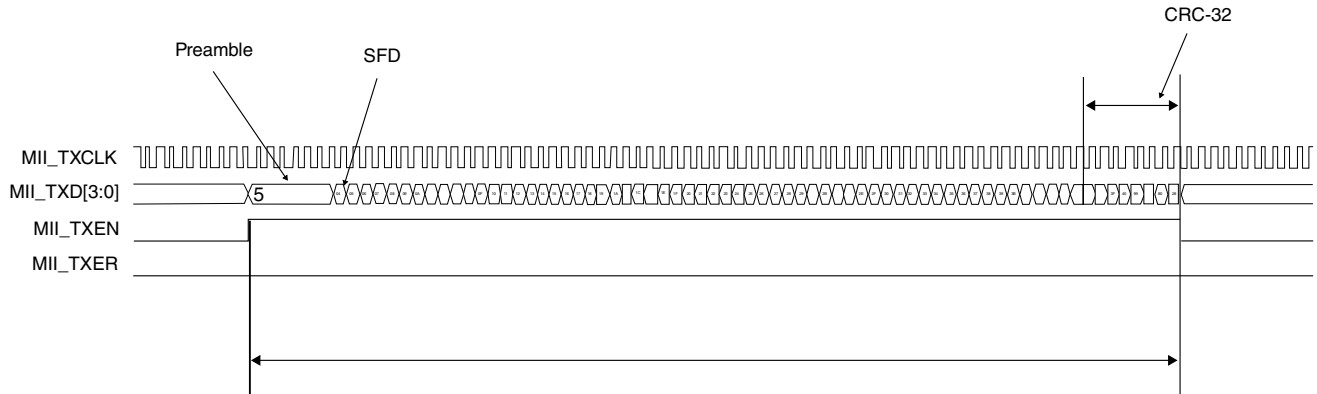
Figure 45-22. MII transmit operation
