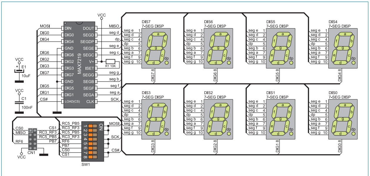
Figure 2: Serial 7-Seg Display 2 additional board connection schematic
