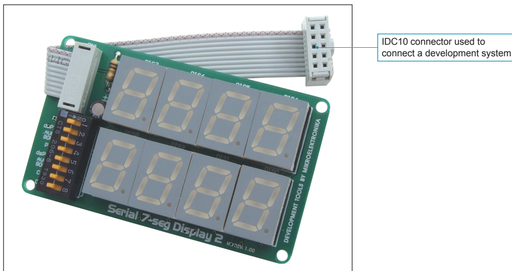
Figure 1: Serial 7-Seg Display 2 additional board
