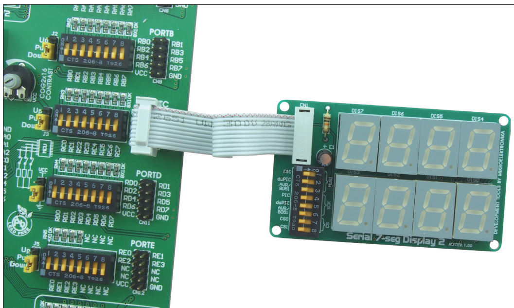
Figure 3: Serial 7-Seg Display 2 additional board connected to a development system
