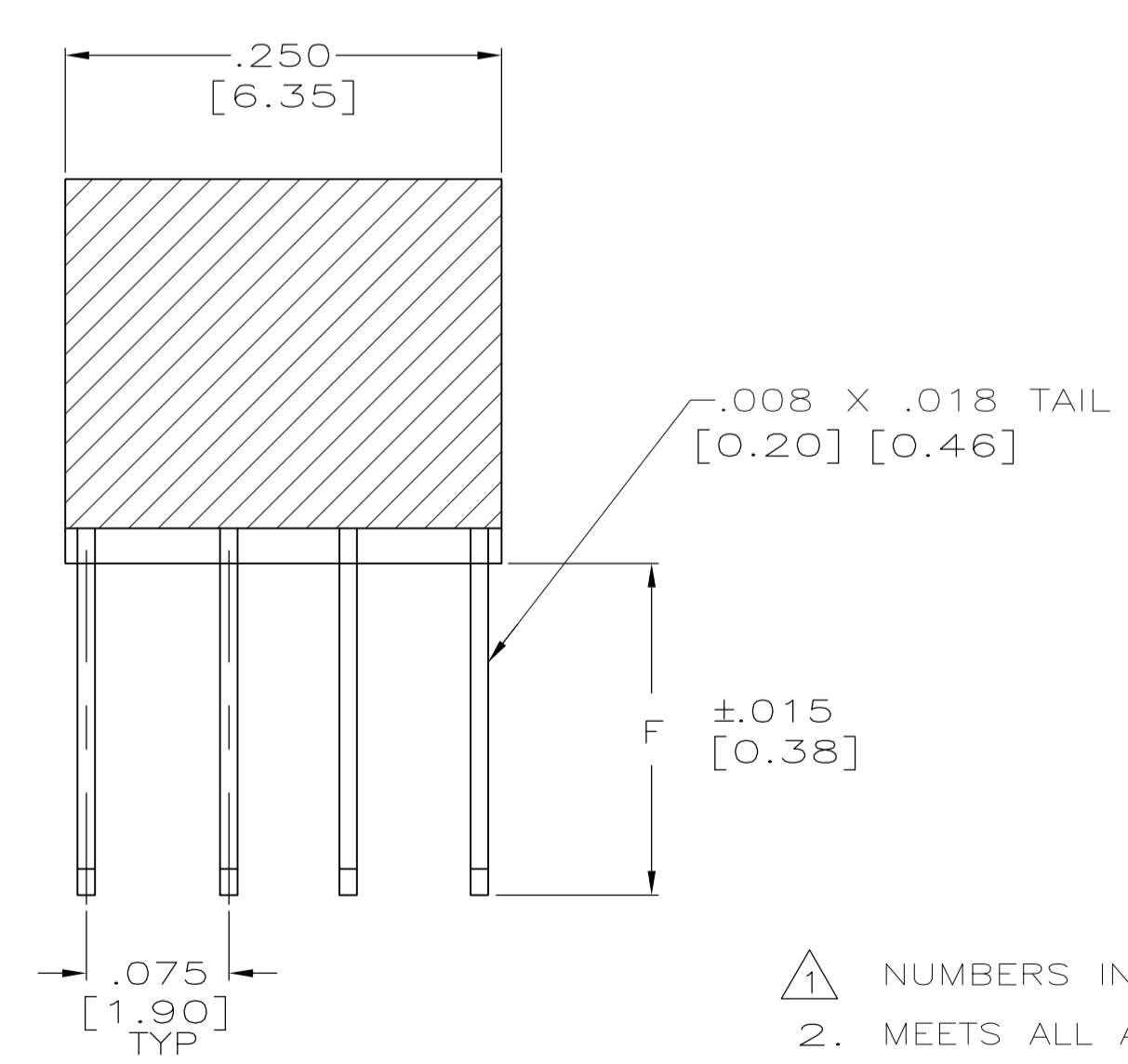
SECTION Z-Z SCALE 10:1
