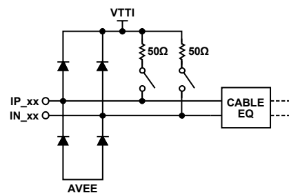
Figure 19. High Speed Input Simplified Schematic
