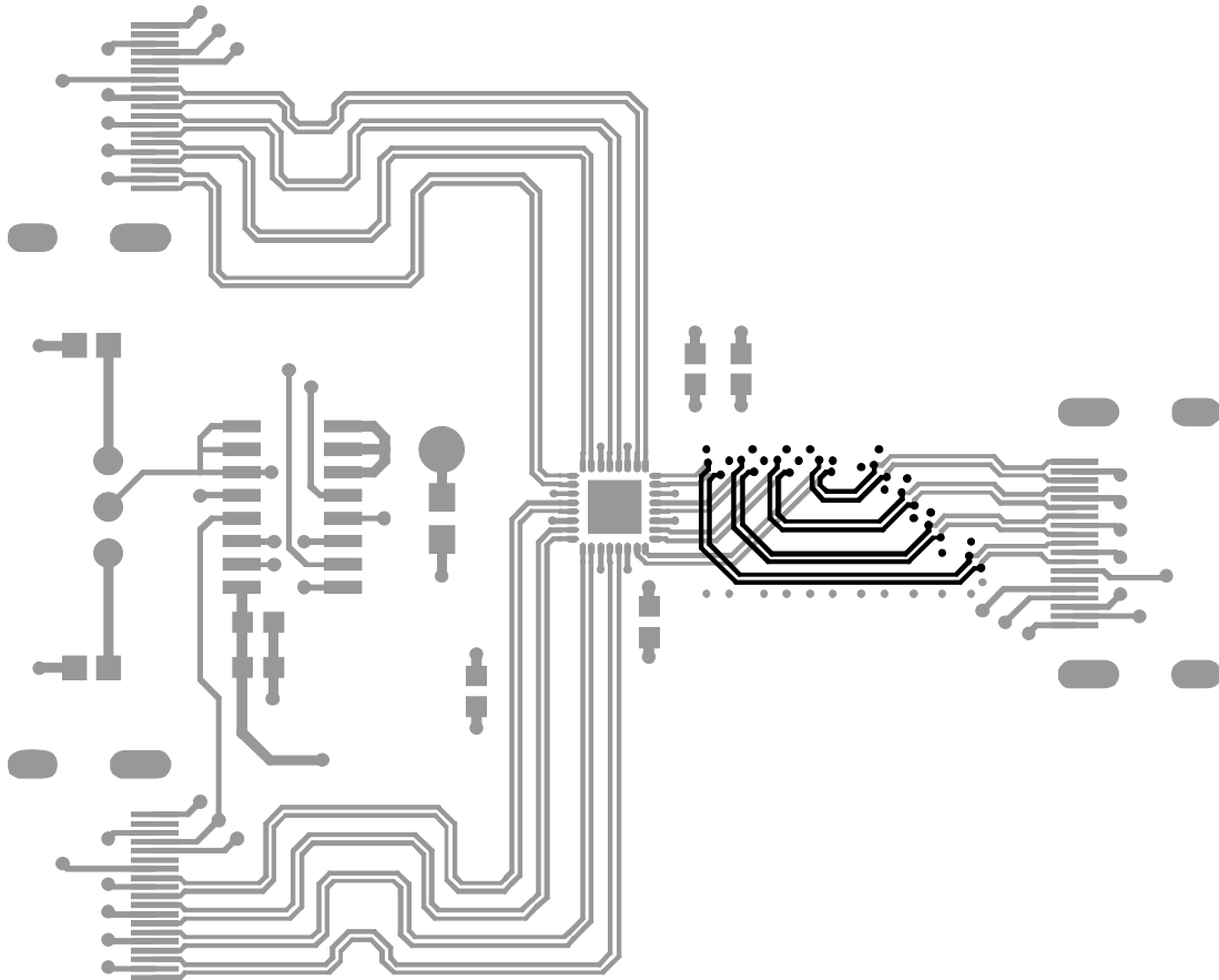
Figure 26. Layout of TMD5 Traces
