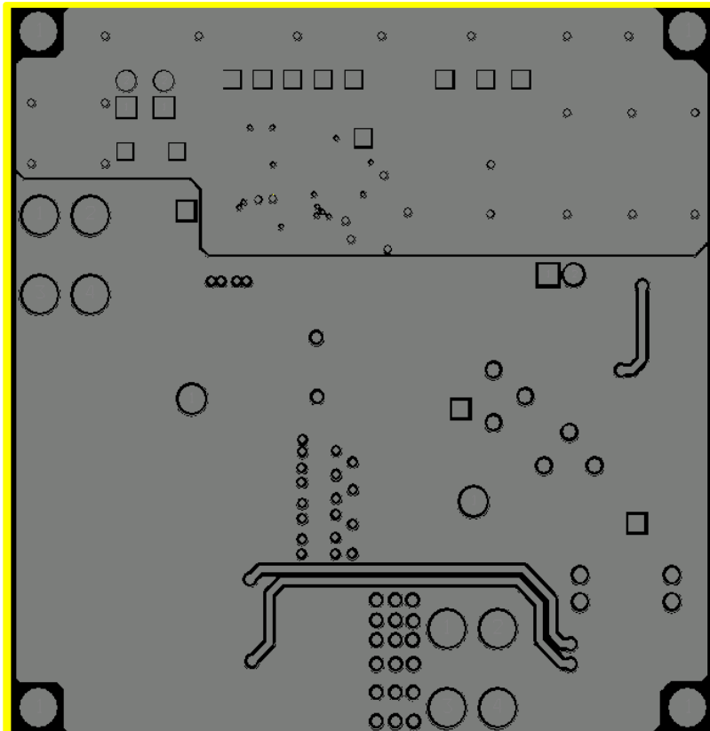
Figure 24. Evaluation Board Inner Layer 1 Copper
