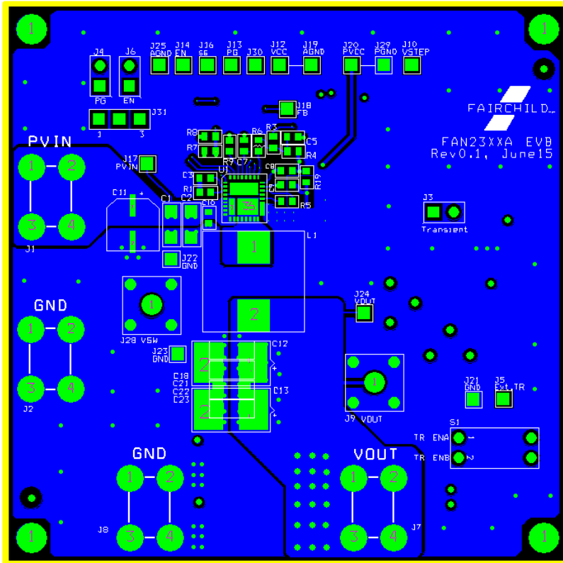
Figure 23. Evaluation Board Top Layer Copper
