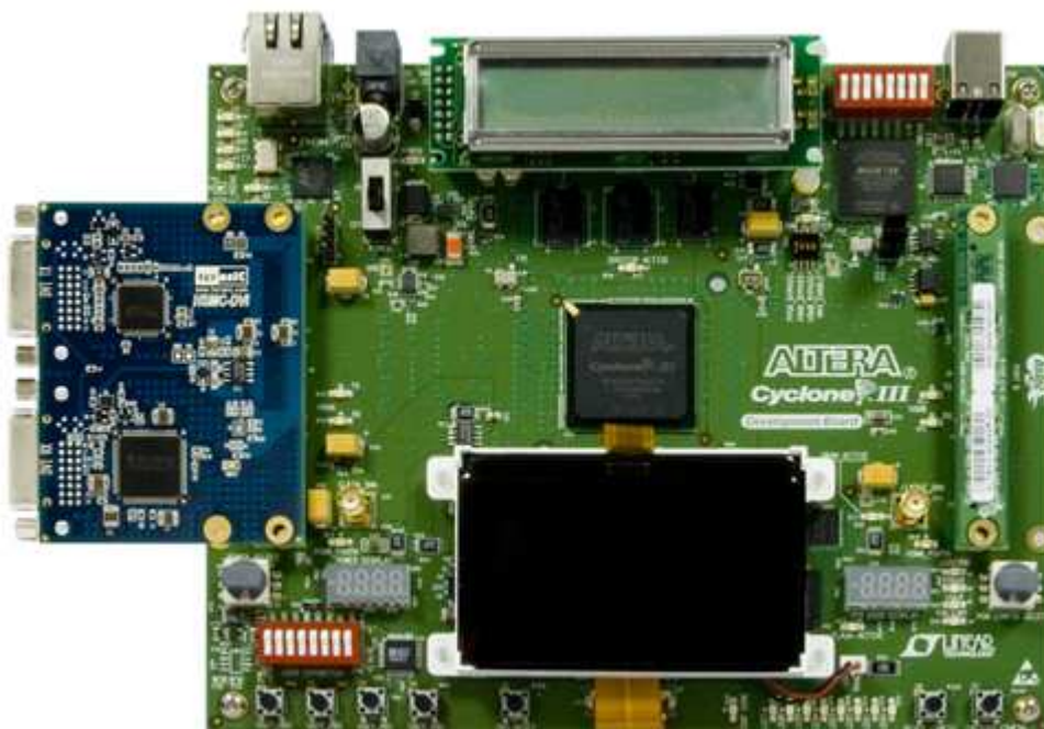
Figure 1.2.4 The HSMC-DVI board connects with Cyclone III Development Board
