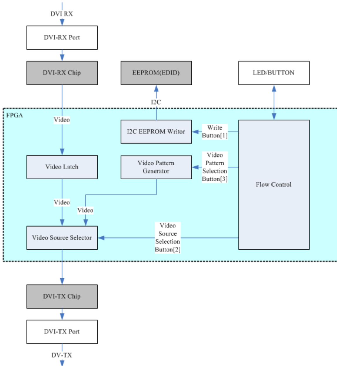
Figure 4.5.1 Block diagram
