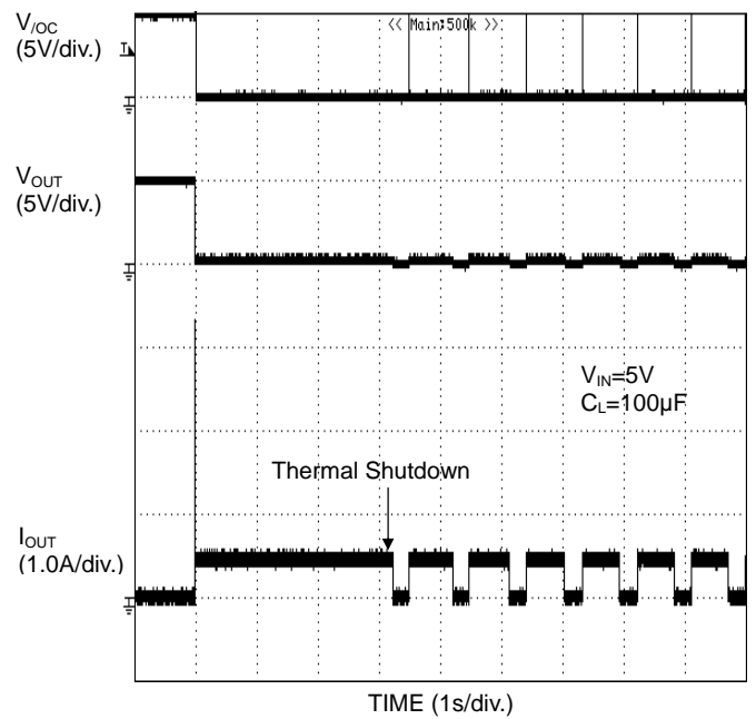
Figure 33. Over current response Enable to short-circuit (BD2045AFJ)
