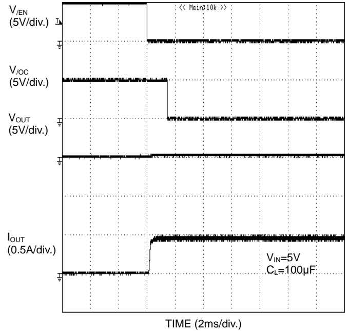
Figure 31. Over current response Enable to short-circuit (BD2045AFJ)
