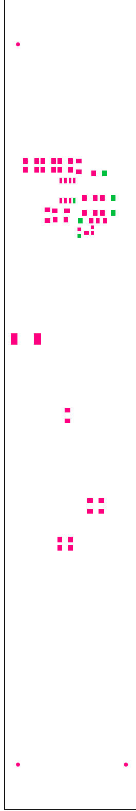
Figure 7. Solder Paste Mask (Bottom)
