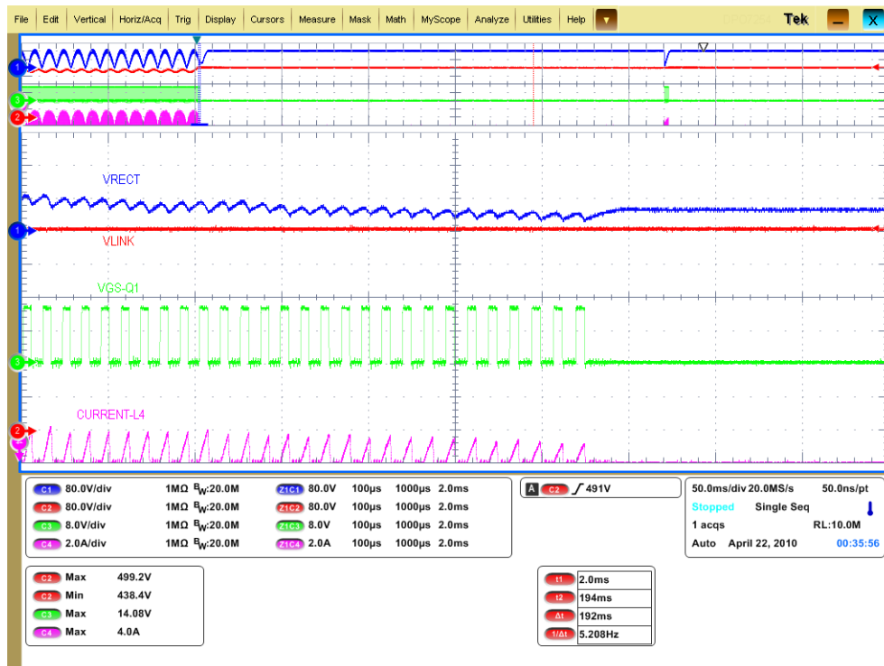
Figure 27. Transient — 115W to Zero Load at 10W/μs, Vin = 120VAC
