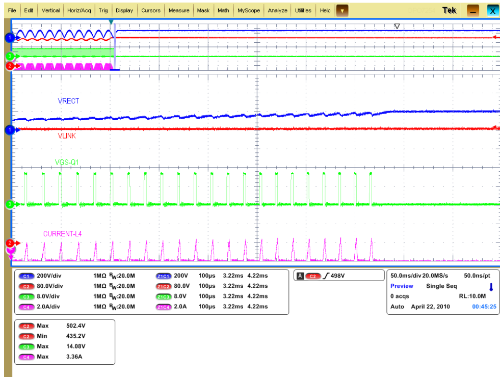
Figure 28. Transient — 115W to Zero Load at 10W/μs, Vin = 230VAC
