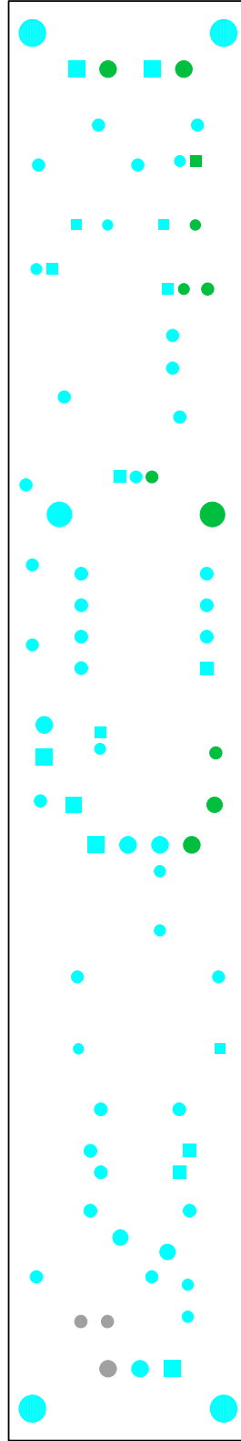
Figure 4. Solder Mask (Top)
