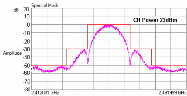
Figure 13. Typical Spectral Plot conforming compliance to IEEE 802.11b 11Mbps CCCK modulation mask at 23dBm output power
