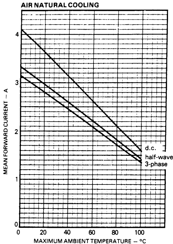
DERATING CURVES
