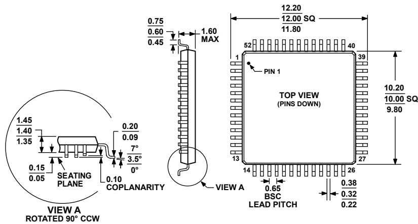
COMPLIANT TO JEDEC STANDARDS MS-026-BCC Figure 32. 52-Lead Low Profile Quad Flat Package [LQFP] (ST-52) Dimensions shown in millimeters
