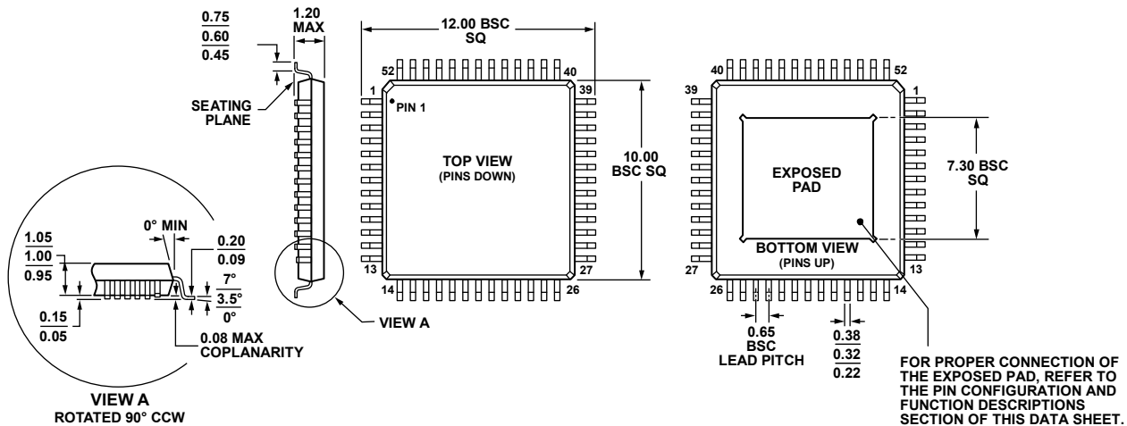
COMPLIANT TO JEDEC STANDARDS MS-026-ACC Figure 33. 52-Lead Thin Quad Flat Package, Exposed Pad [TQFP_EP] (SV-52-2) Dimensions shown in millimeters
